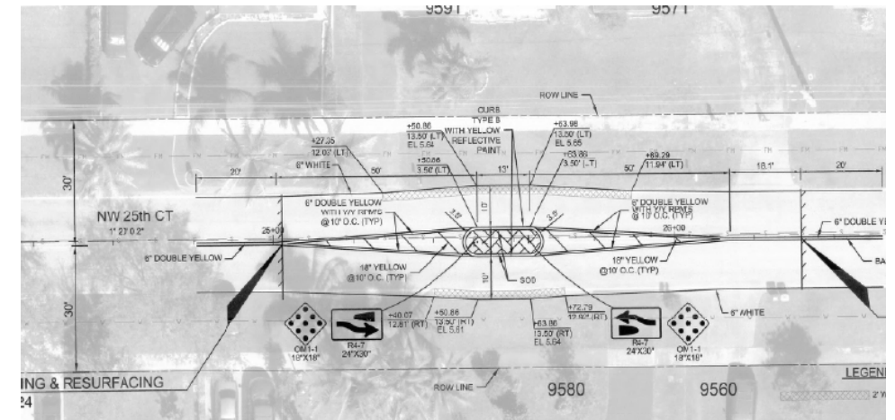
Road Diet Design
