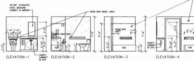
BATHROOM B104
