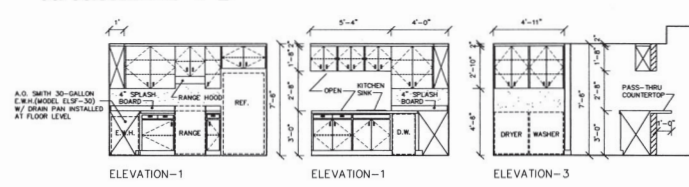
KITCHEN B105
