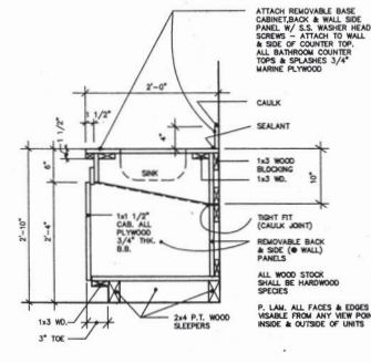
REMOVABLE BASE CAB. DTL.
