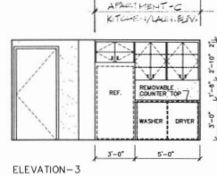
ELEVATION—3
