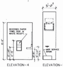
JANITOR
