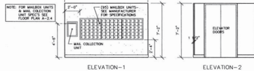
ELEVATOR LOBBY 160
